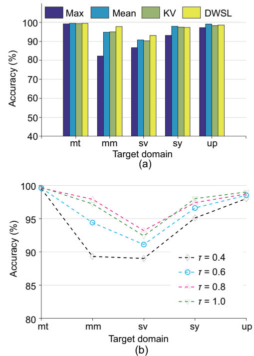
Fig. 2 The accuracy of different pseudo-label strategies in our framework (a) and the sensitivity of hyper-parameter \tau (b)
