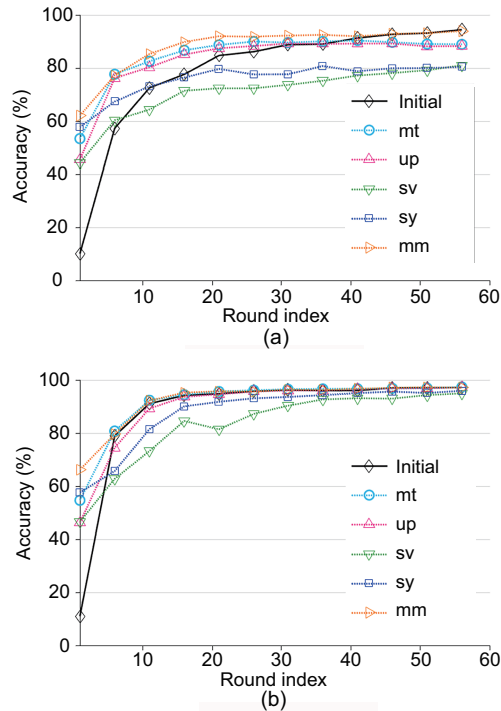
Fig. 3 The accuracy of the local source domain model on the target domain after local training without the collaboration of the local target model (a) and with the collaboration of the local target model by using \ell_{mcr} (b)
