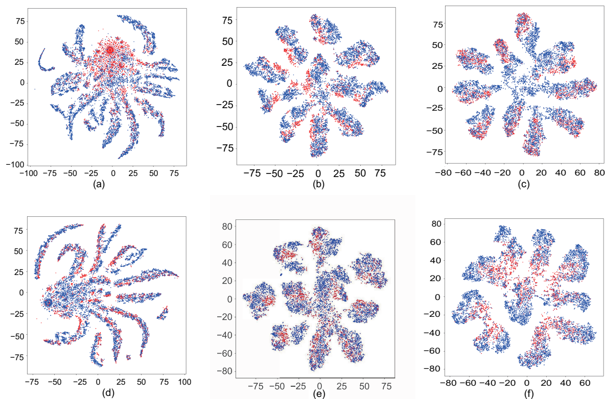
Fig. 4 Visualization of the features (blue points) from the source domains and the features (red points) from the target domain on the Digit-5 dataset
