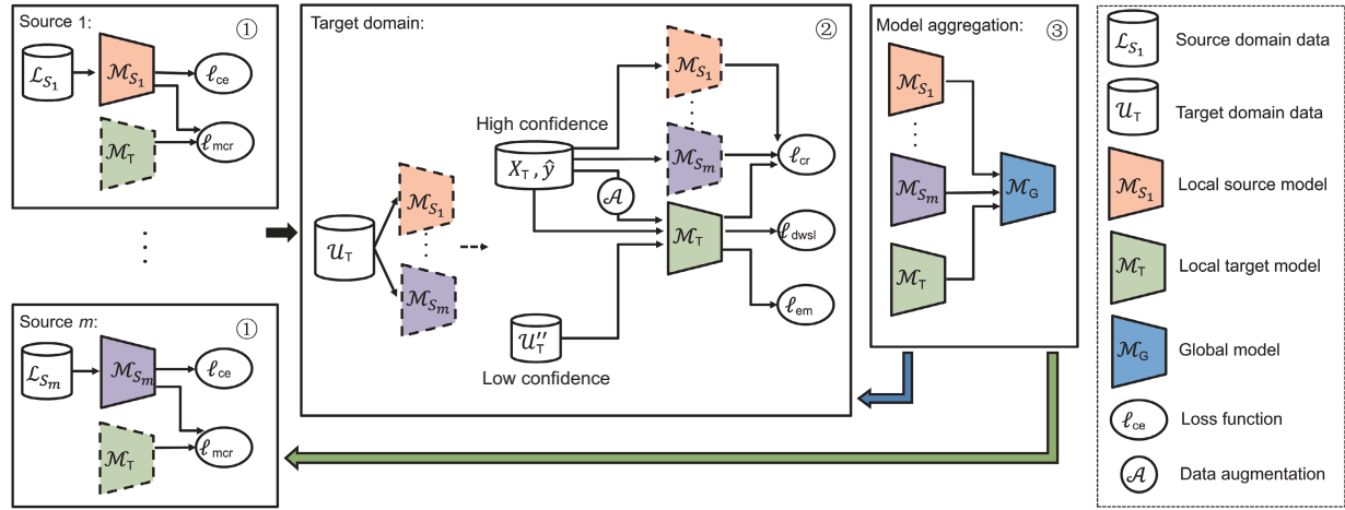
Fig. 1 The framework of dual collaboration decentralized multi-source domain adaptation (DC-MDA) for solving decentralized multi-source domain adaptation (DMDA)
